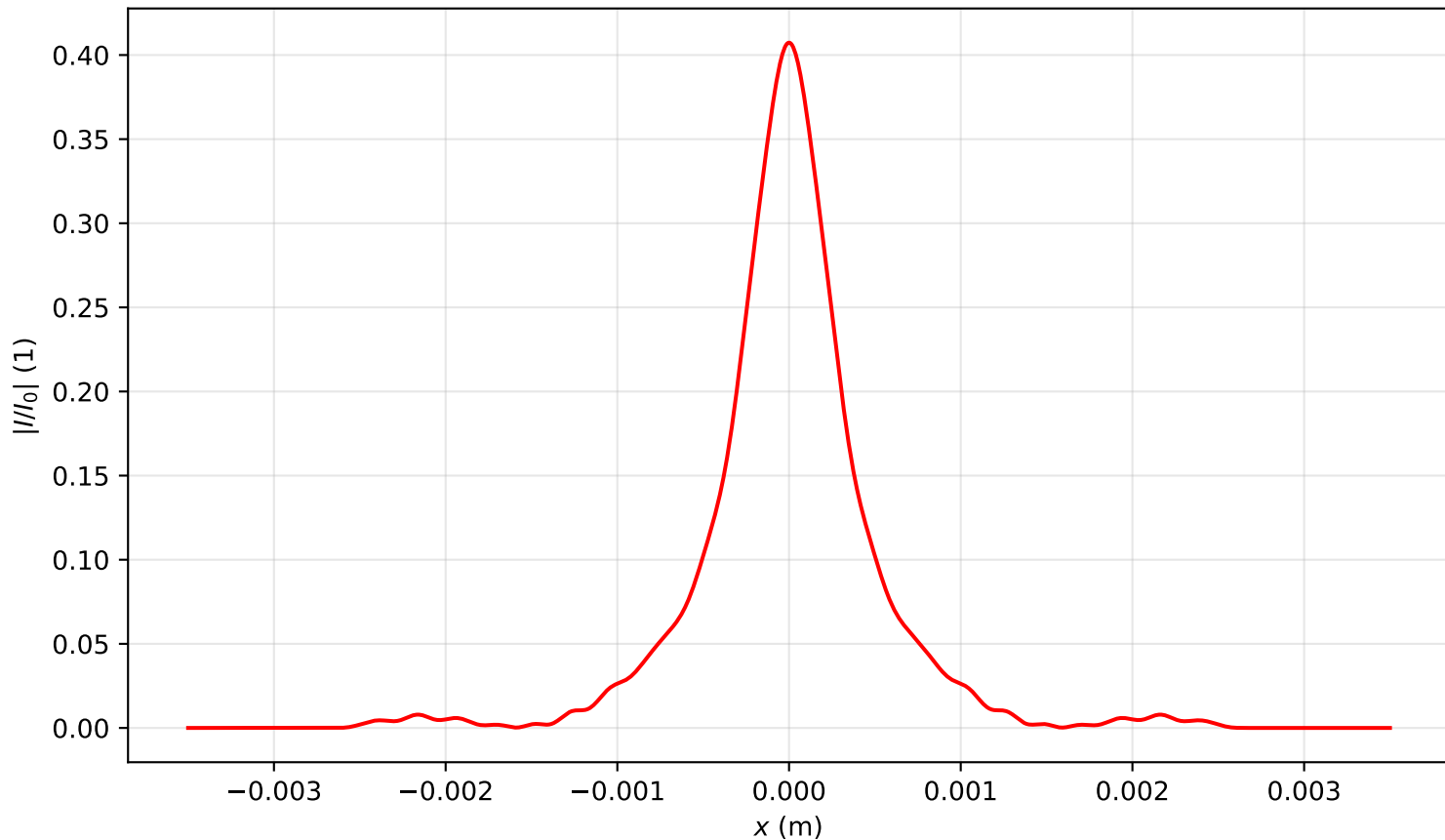
Intensity profile I(x, y = 0, z = 1.592)/I_0 , P_{in}=3.0P_{cr} , artificial time
